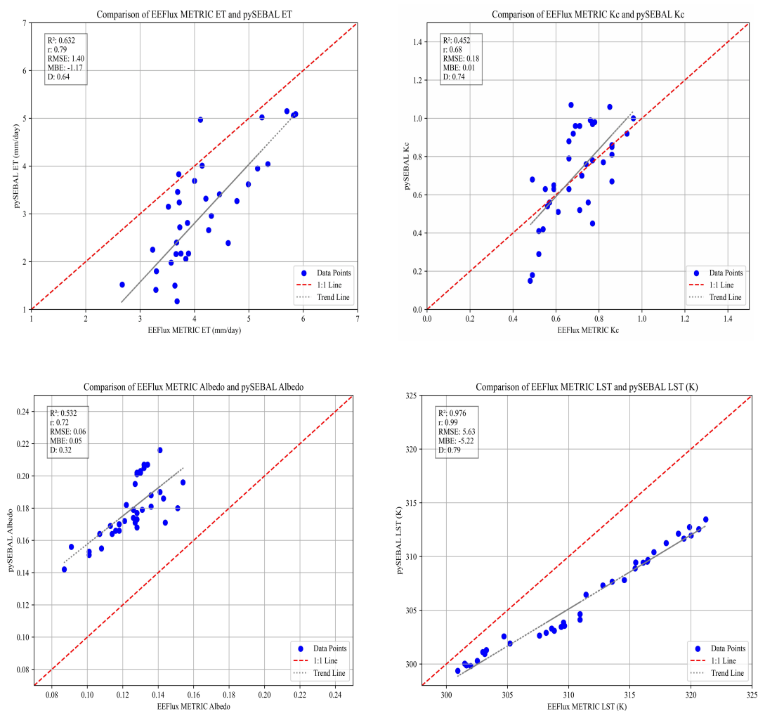
Fig. 2. Statistical comparison between SEBAL and EEFlux METRIC model parameters.
